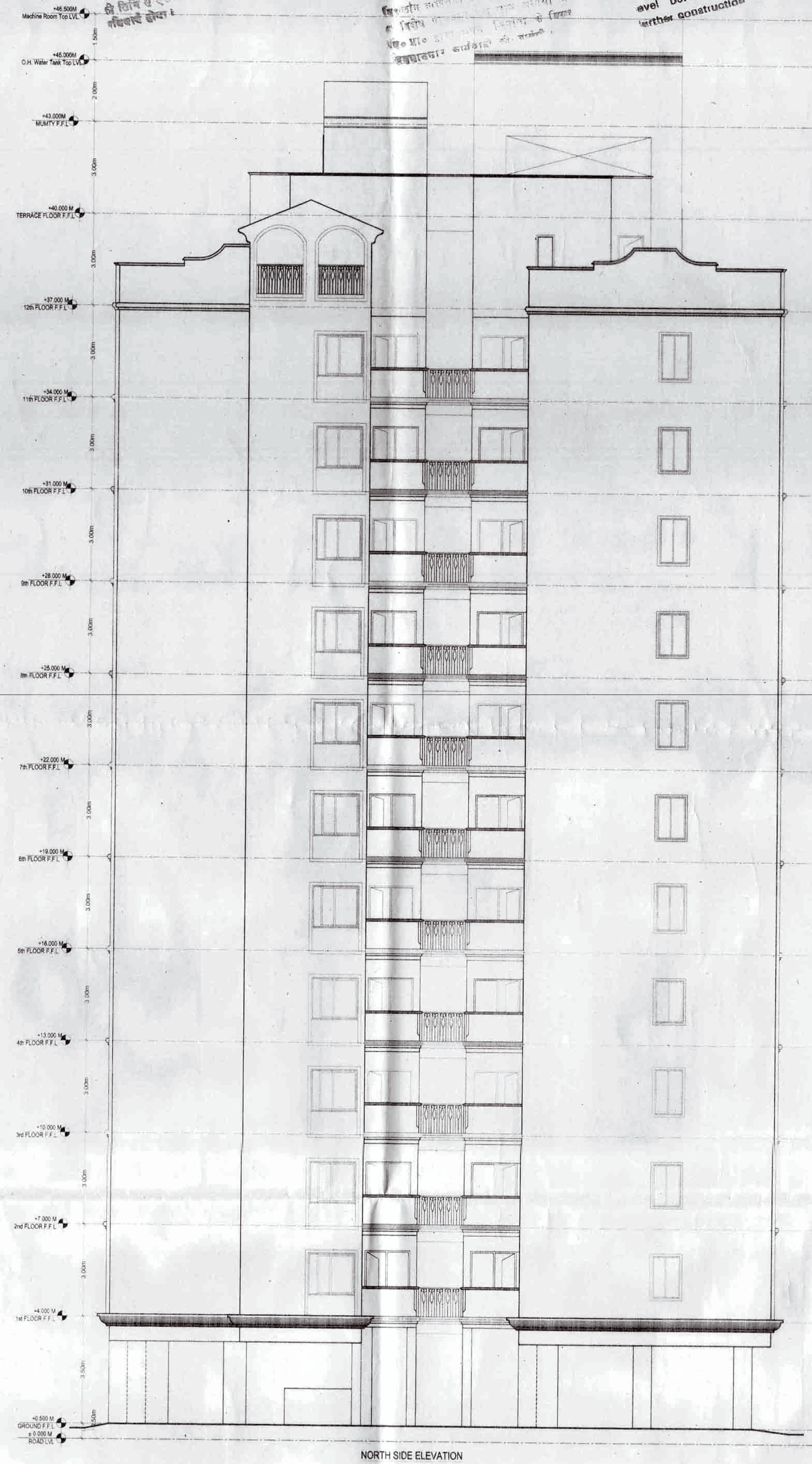
NORTH SIDE ELEVATION
